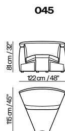
45° wedge corner
