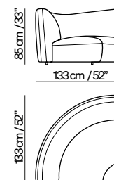
round corner
