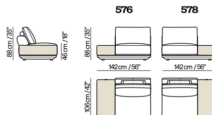
chair with integrated tabletop
