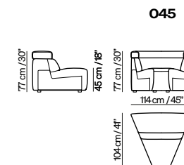
45° wedge corner
