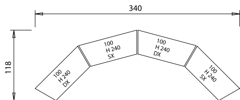
Comp. 3 340 x 118 x h 240 2 x 100 h 240 dx + 2 x 100 h 240 sx
