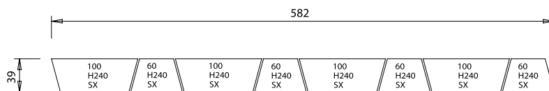
Comp. 4 582 x 39 x h 240 4 x 100 h 240 sx + 4 x 60 h 240 sx
