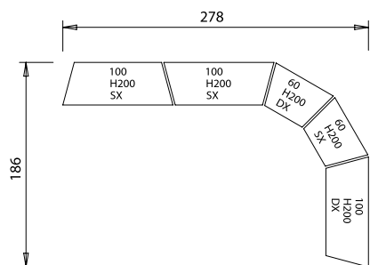
Comp. 1 278 x 186 x h 200 2 x 100 h 200 sx + 1 x 100 h 200 dx 1 x 60 h 200 dx + 1 x 60 h 200 sx
