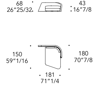
T1-3 seat
