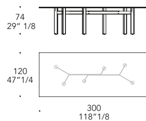
Square-Round 300
