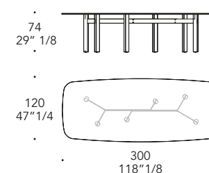
Square-Round 300
