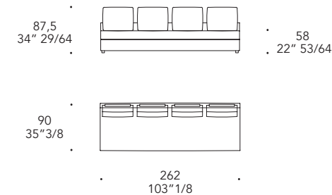
E - 4 seats element
